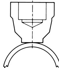
Non-Pilot Boss, Class 400. Socket Weld
