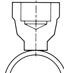
Pilot Boss, Class 400 Socket Weld
