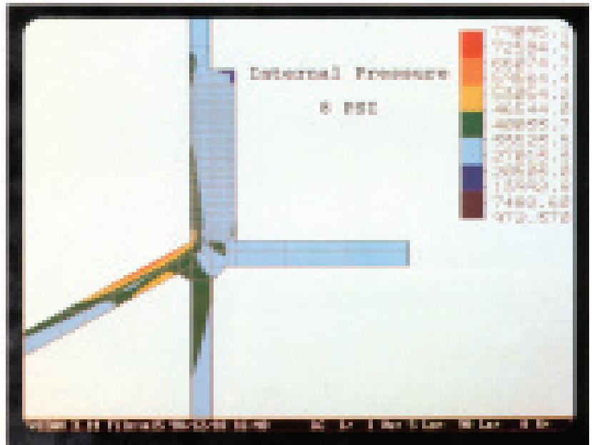
A portion of a pressure vessel with its stress pattern displayed by a finite element analysis. This method can calculate stresses for design details not covered by ASME Code or TEMA rules.
